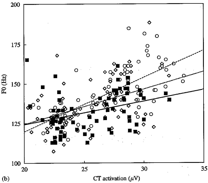
Figure 1. Plots of CT activation by F0 for the three vowels, plotted separately for each subjects: (a) M1, left. (b) M1, right. (c) M2. (d) W1. (e) W2: —, ■ F0-a; ·····, ◇ F0-i; ----, ○ F0-u.
